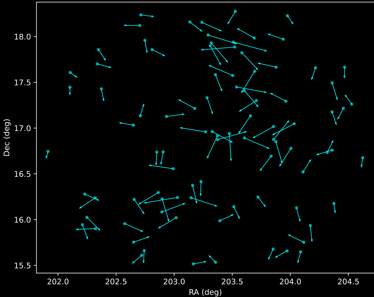
APOGEE DR17 Noise Stream Proper Motion Vectors (n=91)
