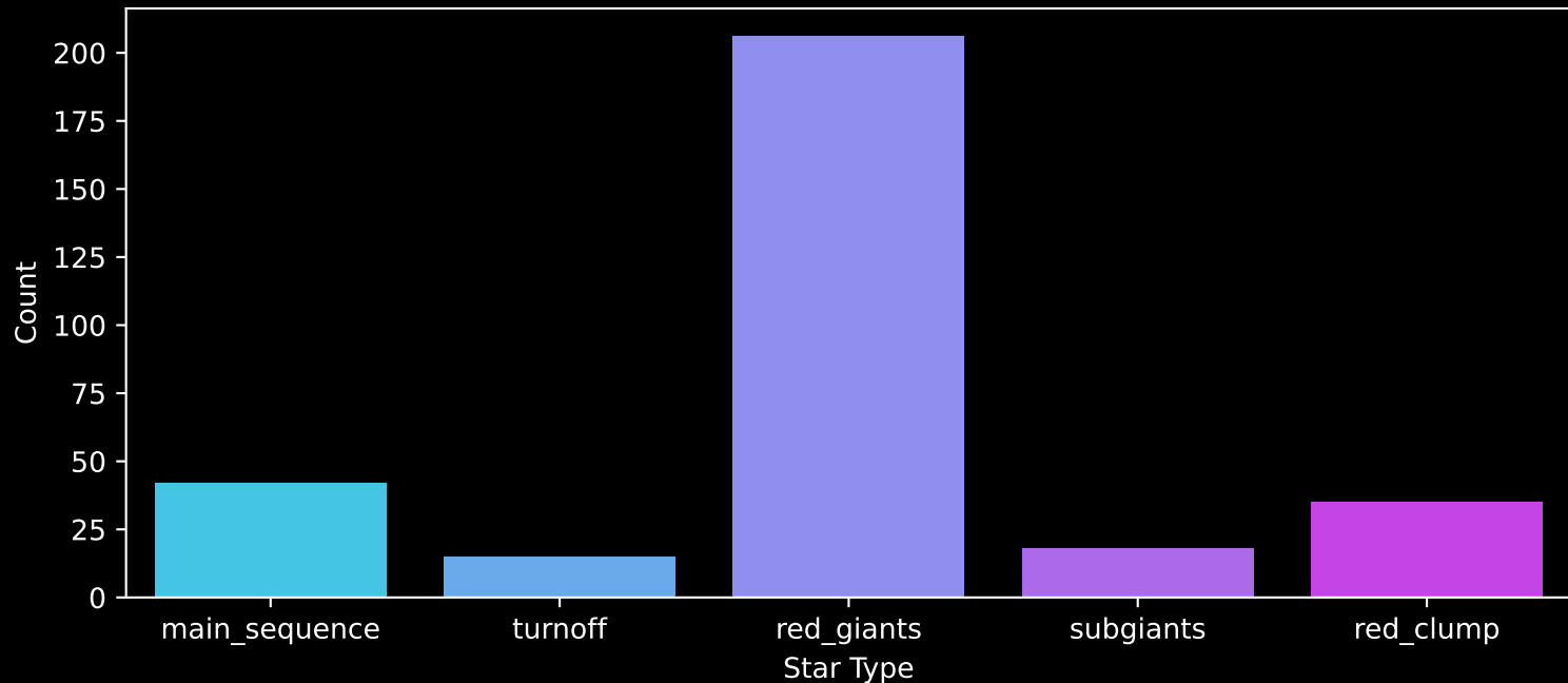
APOGEE DR17 Field: [198+08] Count plot of Star Type
