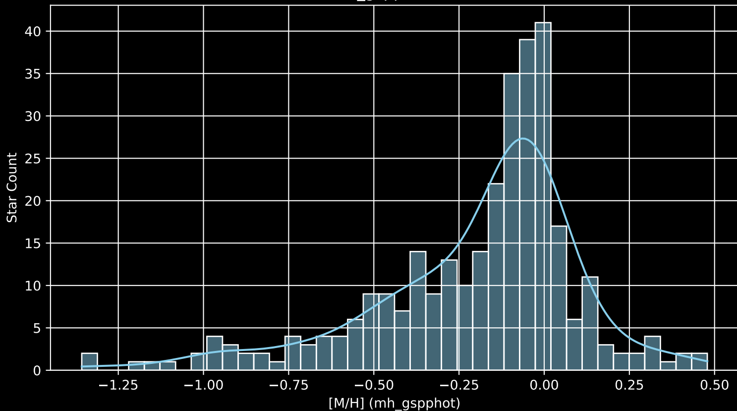
APOGEE DR17 Field: [198+08 [M/H] (mh_gspphot) (n= 312)
