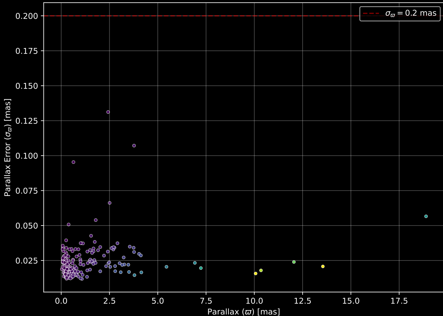
APOGEE DR17 Field: [198+08] Parallax Quality (n= 316)
