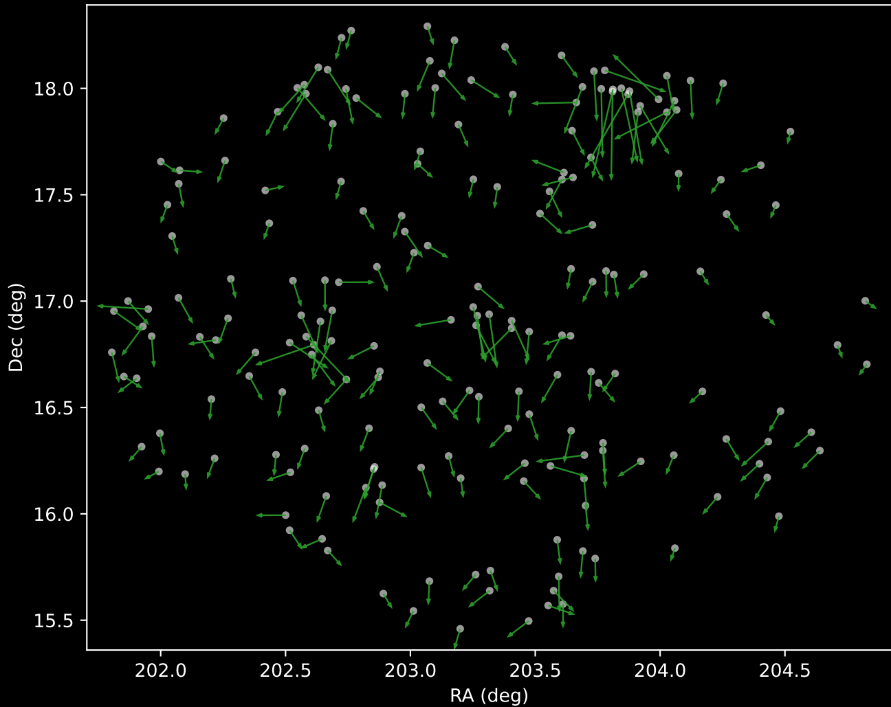
APOGEE DR17 Cluster 4 Proper Motion Vectors (n=200)
