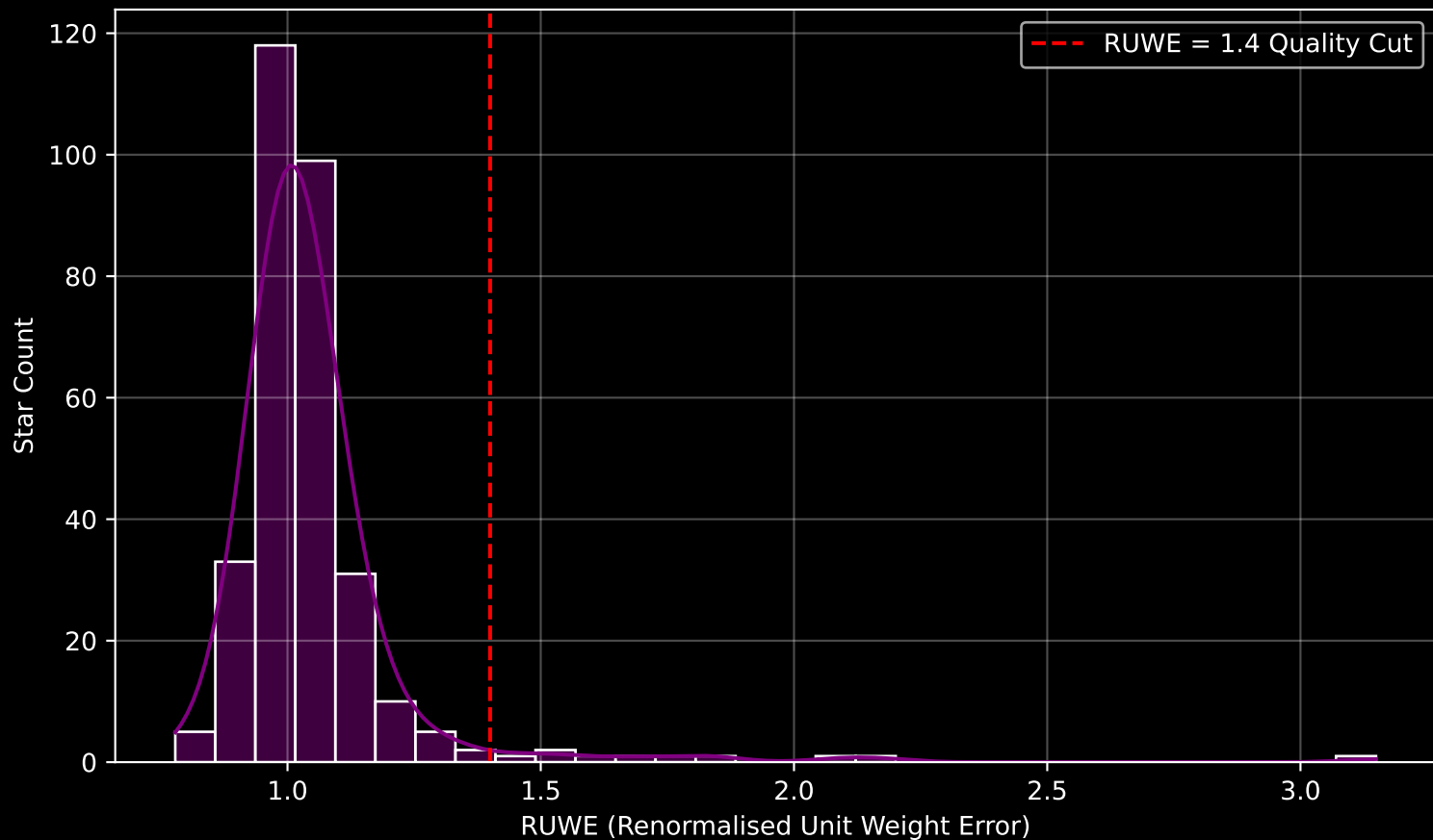
GAPOGEE DR17 Field [198+08] RUWE Distribution (n= 313)
