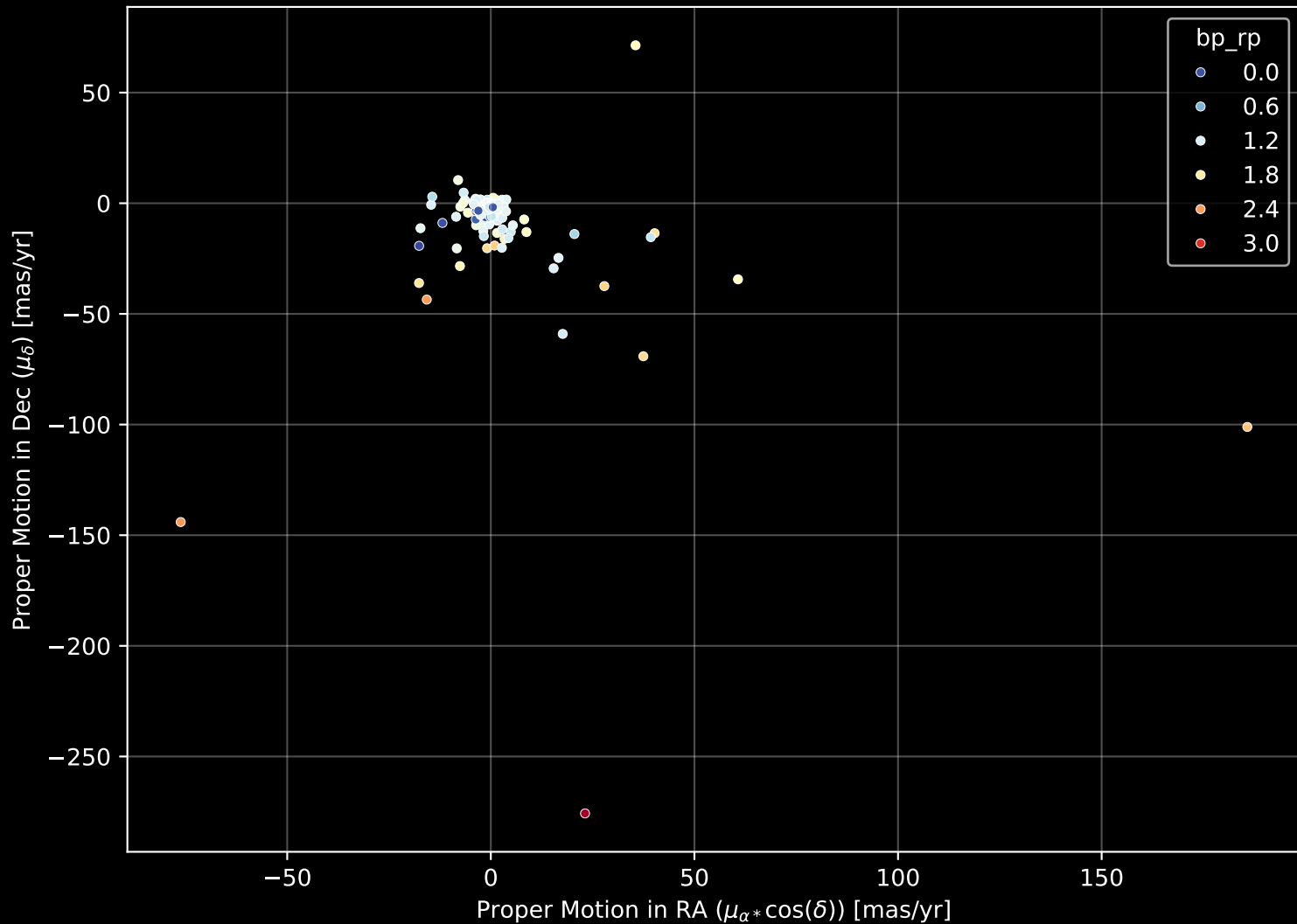
APOGEE DR17 Field: [198+08] Proper Motion Diagram (n= 316)
